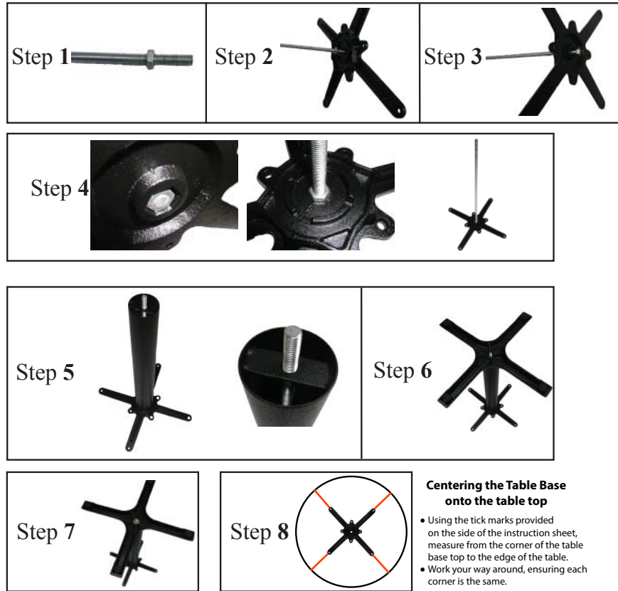
Assembly Illustration
